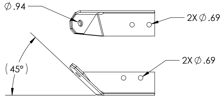
DETAIL -A- SCALE 1:8
